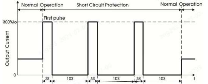
Short circuit protection curve (Typ.)
