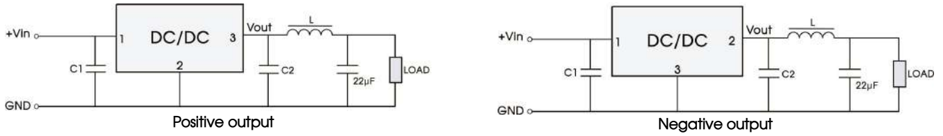
Fig. 4 Using the "LC" output filter application
