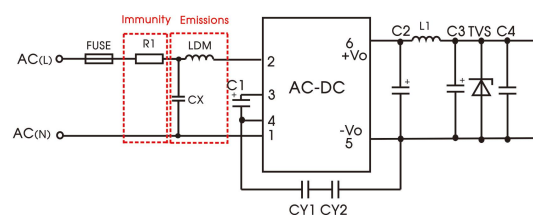
Recommended circuit 2
