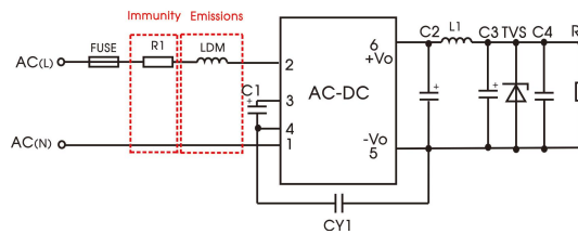
Recommended circuit 1
