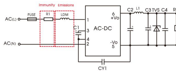
recommended circuit 1
